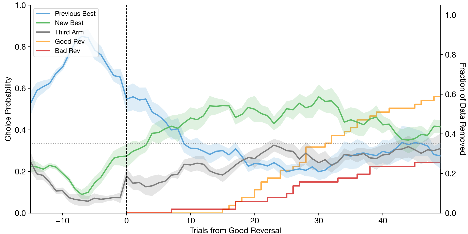
Good Reversal-Aligned Choices (mean \pm se across subjects | n=6 subjects, n=51 reversals)
